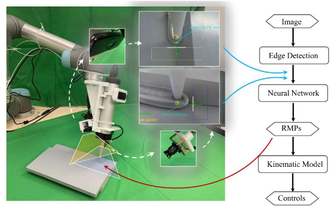
Fig. 2. Overview of the neural path planning framework with RMPs for automatic robotic sealing. The interaction between the sealing gun and the workpiece environment is modeled with neural RMPs. Typically, the interaction could be attractive (yellow), and the heading correction (green). The RMPs are predicted by training a neural network with the ROI features from two different camera views. The RMPs are then combined into the forward kinematics of the robotic sealing system to solve the control commands. (For interpretation of the references to color in this figure legend, the reader is referred to the web version of this article.)
