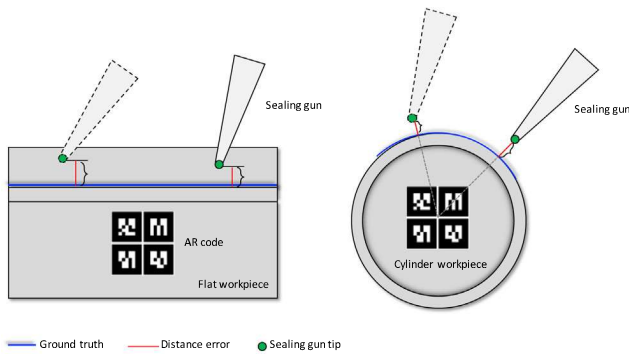
Fig. 14. Conceptual representation of the distance error computation on two selected workpieces in reactive path planning experiments. (For interpretation of the references to color in this figure legend, the reader is referred to the web version of this article.)
